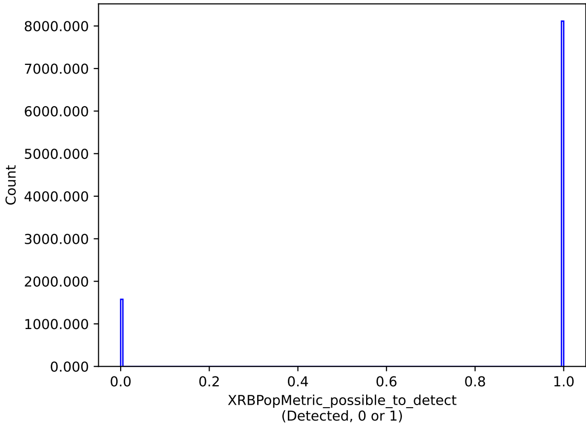
early_u_fpextra2.0_v3.4_10yrs : XRBPopMetric_possible_to_detect
