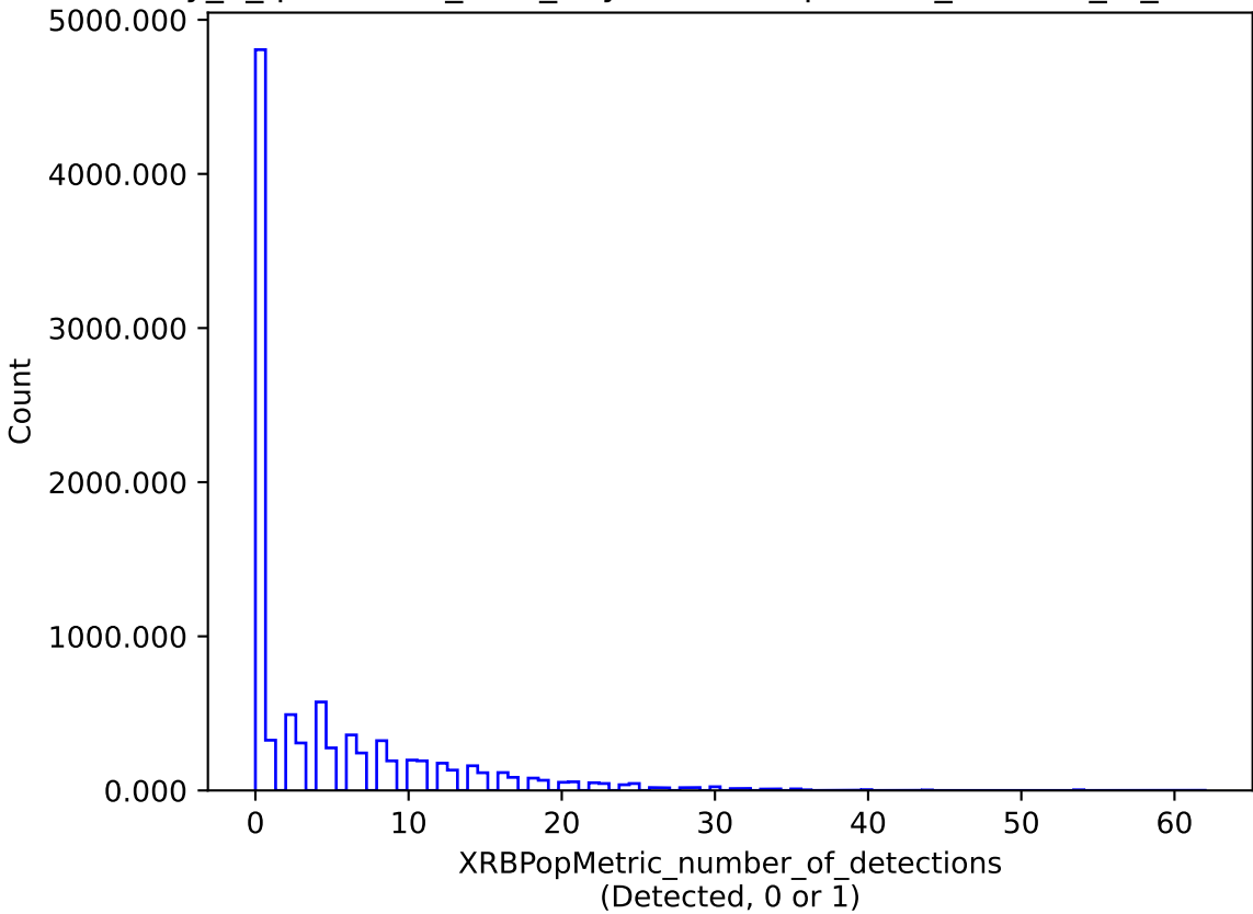
early_u_fpextra2.0_v3.4_10yrs : XRBPopMetric_number_of_detections
