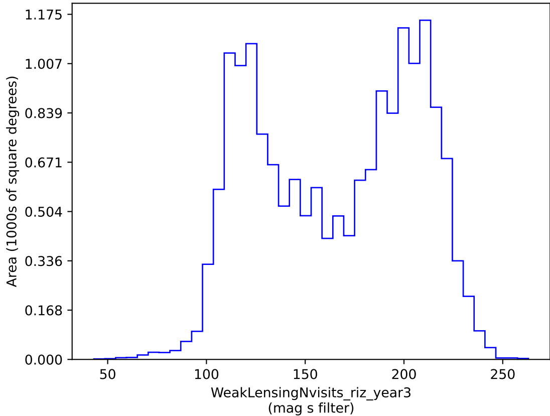
early_u_fpextra2.0_v3.4_10yrs gri band non-DD: WeakLensingNvisits_riz_year3
