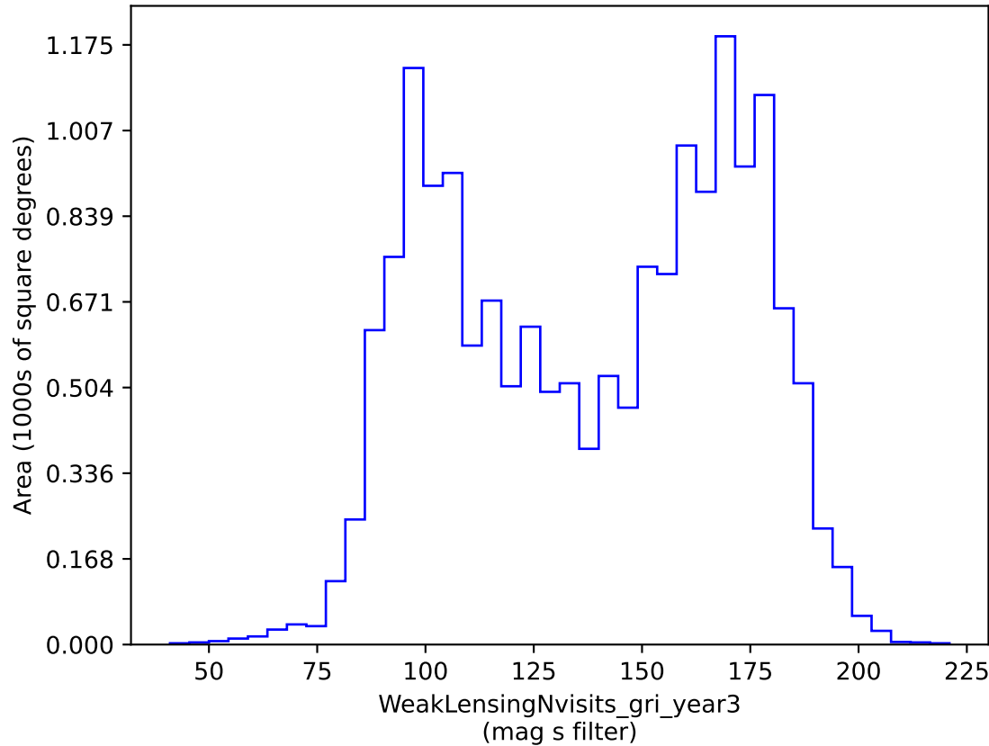
early_u_fpextra2.0_v3.4_10yrs gri band non-DD: WeakLensingNvisits_gri_year3
