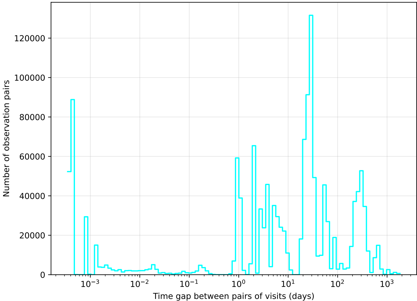
early_u_fpextra2.0_v3.4_10yrs u band: Tgaps observationStartMJD
