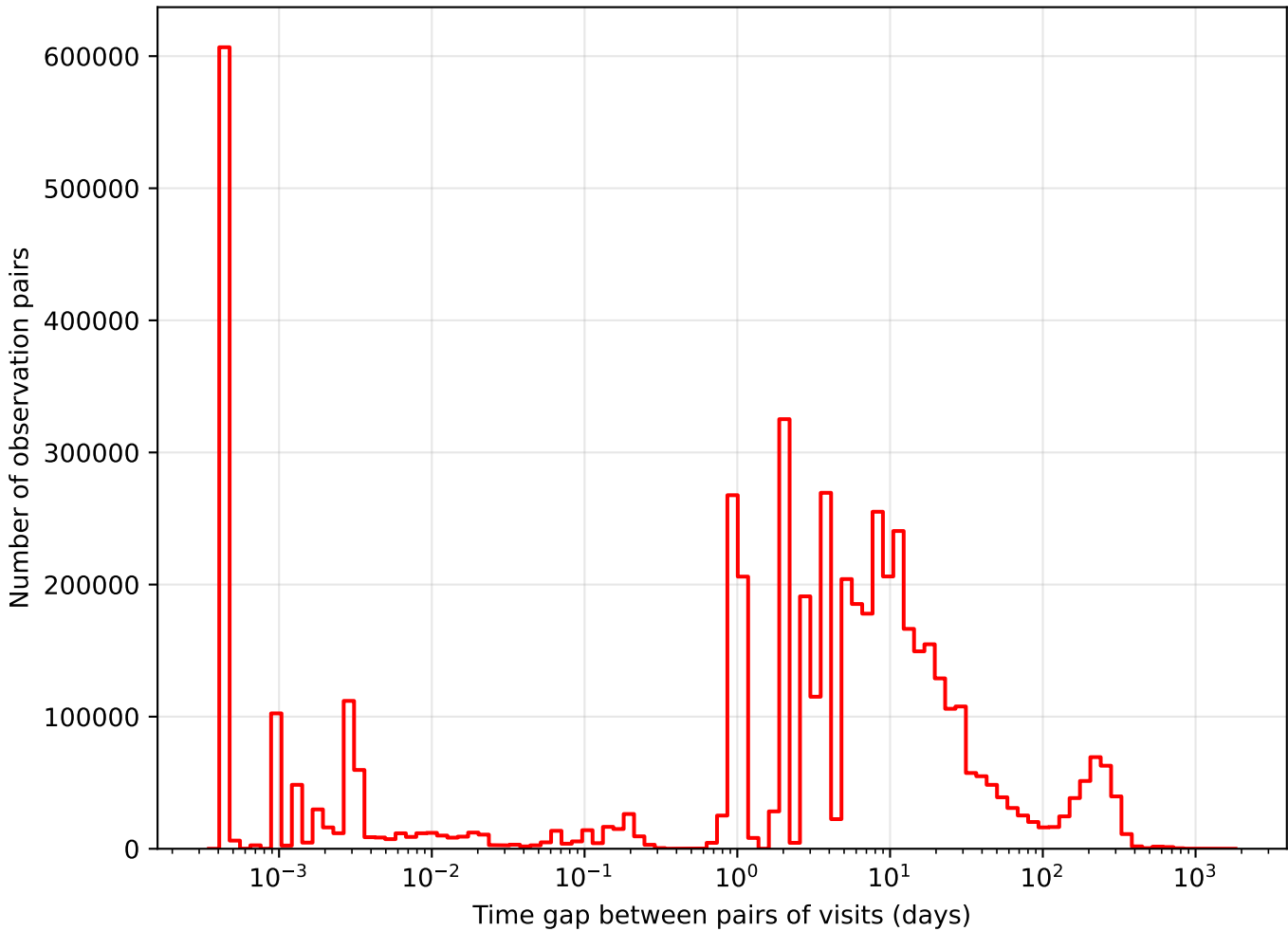
early_u_fpextra2.0_v3.4_10yrs i band: Tgaps observationStartMJD
