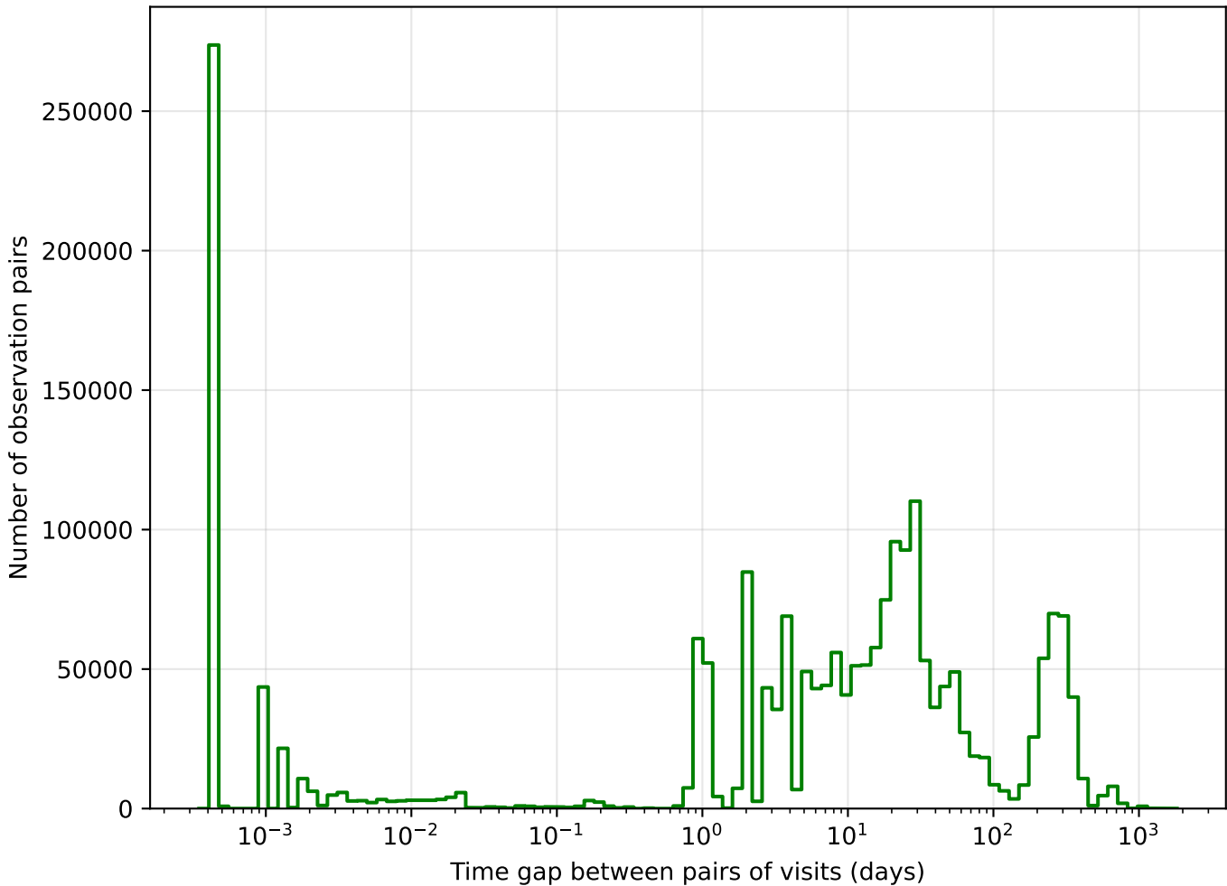
early_u_fpextra2.0_v3.4_10yrs g band: Tgaps observationStartMJD
