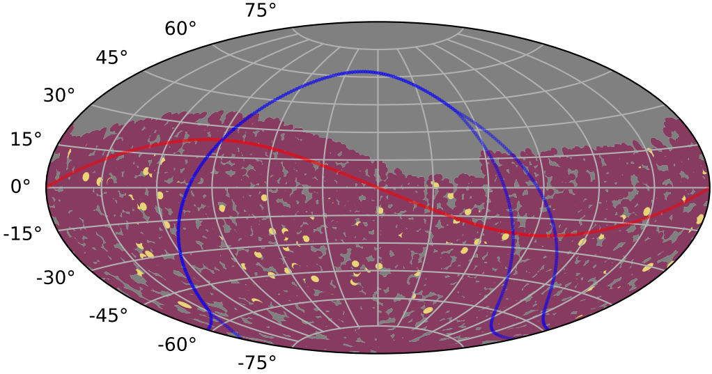
early_u_fpextra2.0_v3.4_10yrs : TDEsPopMetric_some_color_pu
