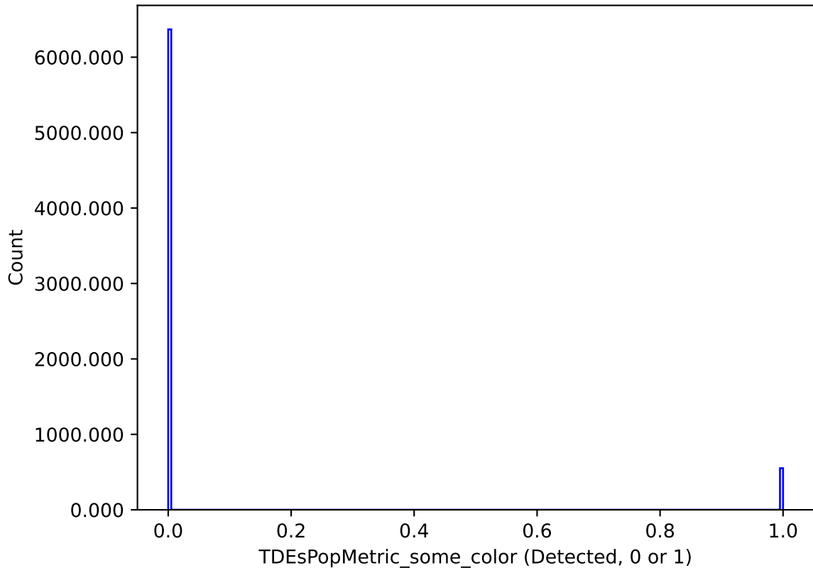
early_u_fpextra2.0_v3.4_10yrs : TDEsPopMetric_some_color
