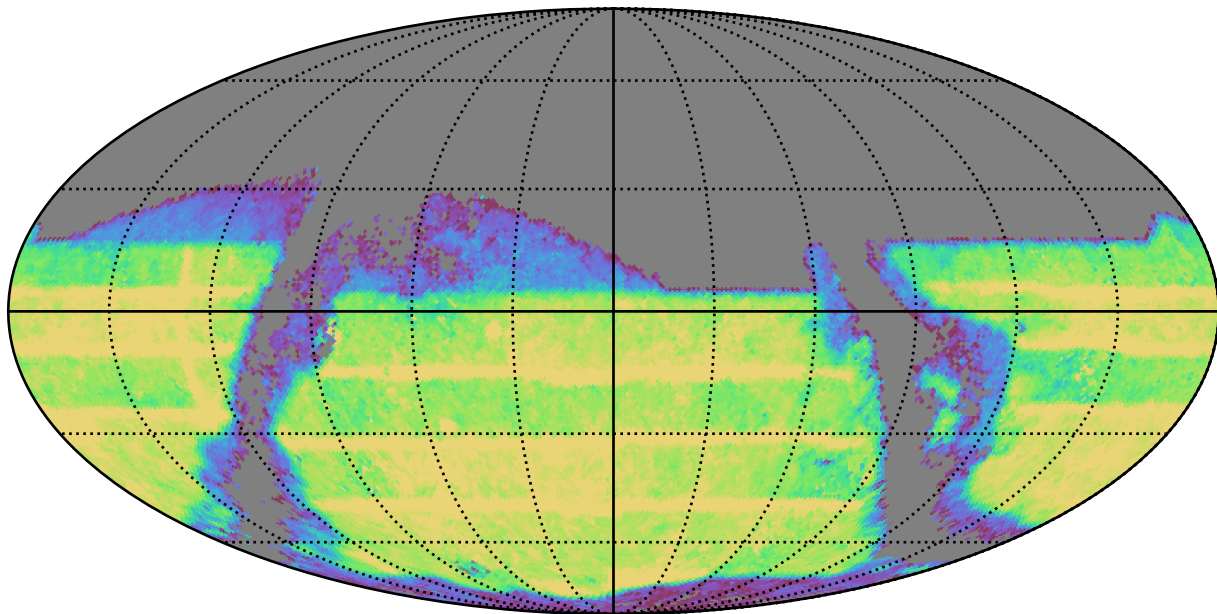
early_u_fpextra2.0_v3.4_10yrs : TDC_rate
