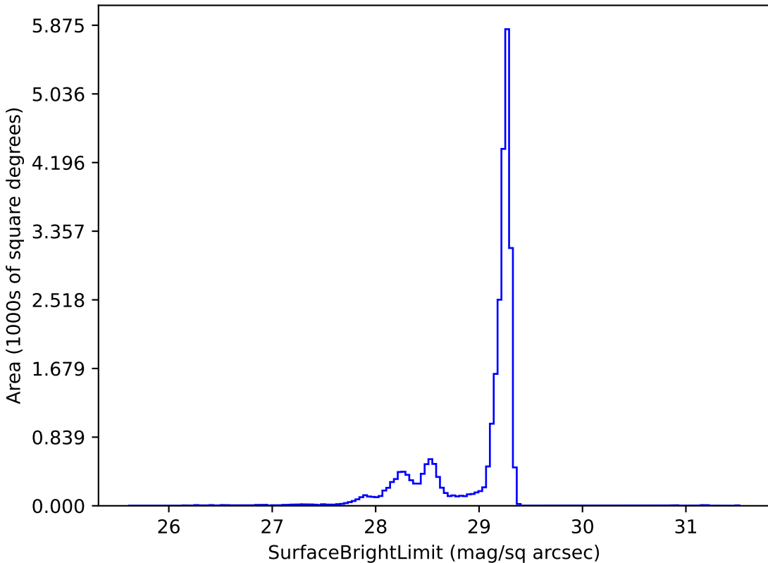
early_u_fpextra2.0_v3.4_10yrs z: SurfaceBrightLimit
