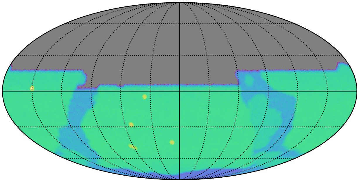
early_u_fpextra2.0_v3.4_10yrs y: SurfaceBrightLimit
