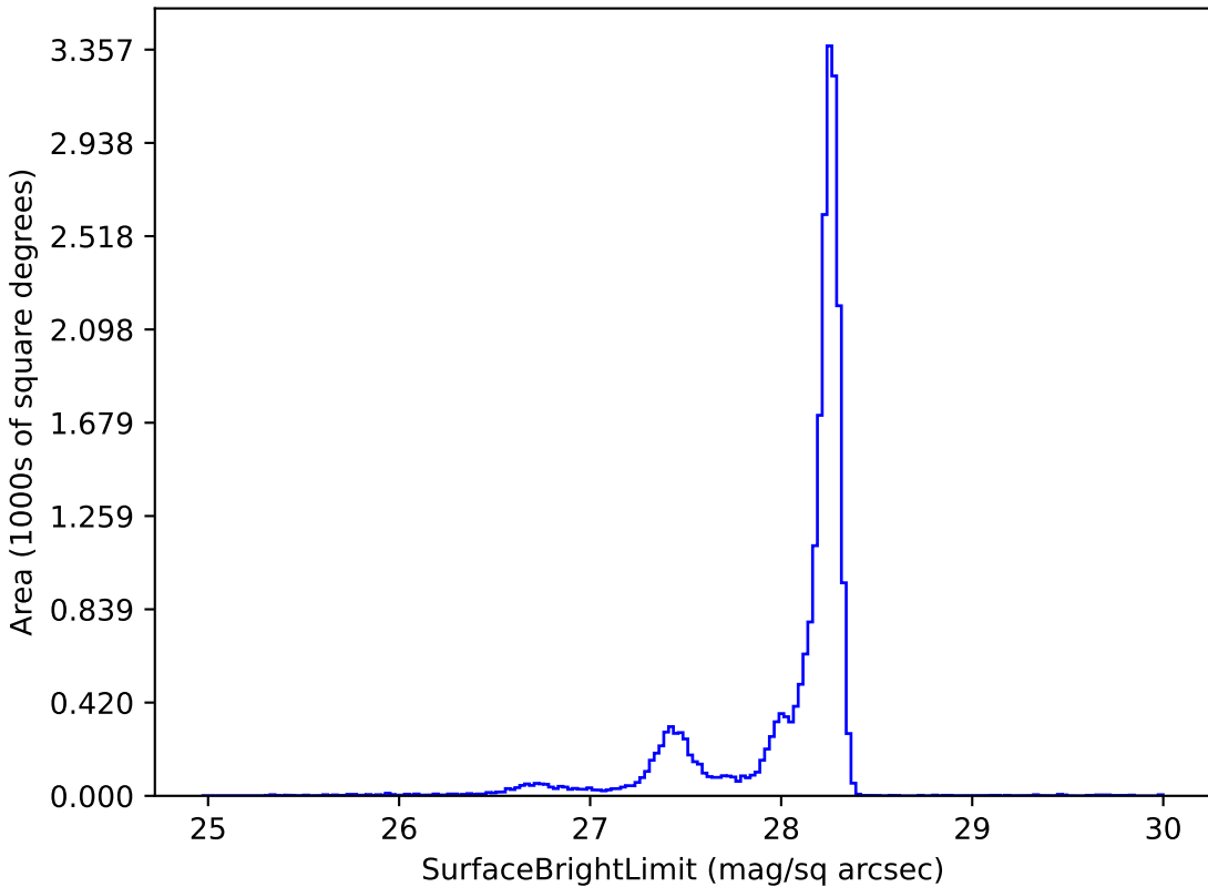
early_u_fpextra2.0_v3.4_10yrs y: SurfaceBrightLimit
