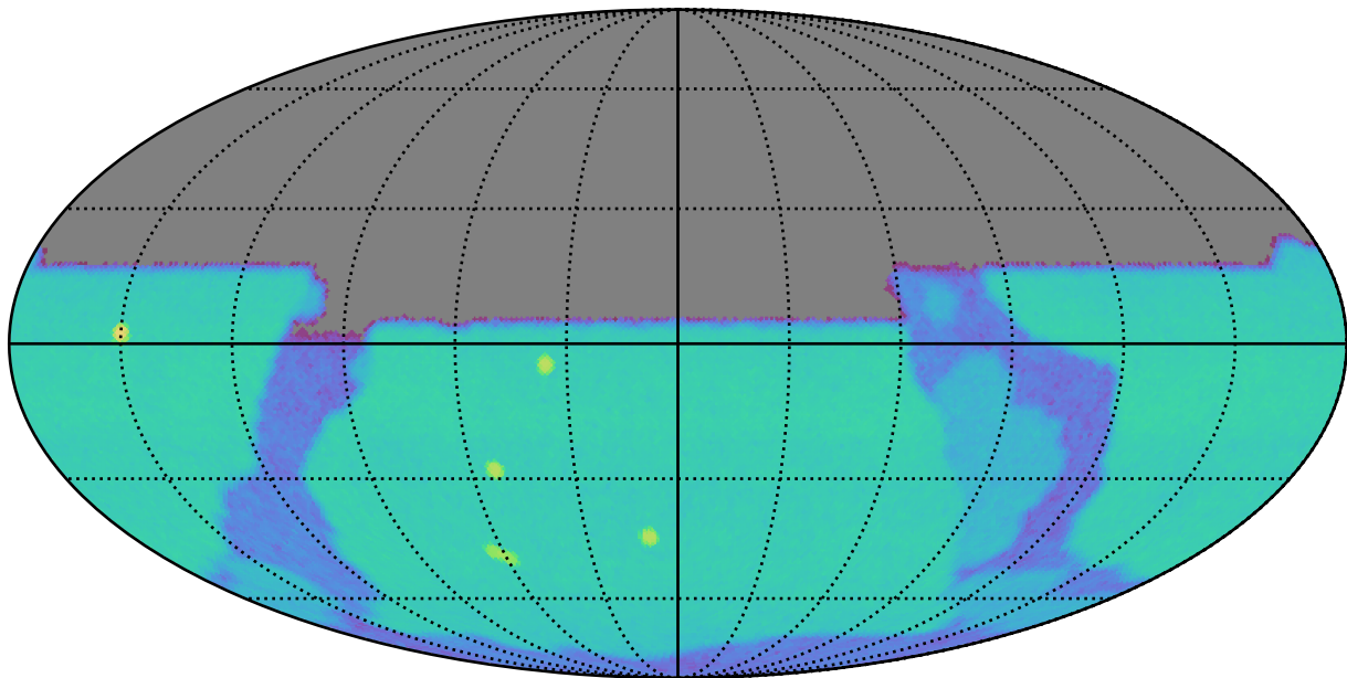
early_u_fpextra2.0_v3.4_10yrs u: SurfaceBrightLimit
