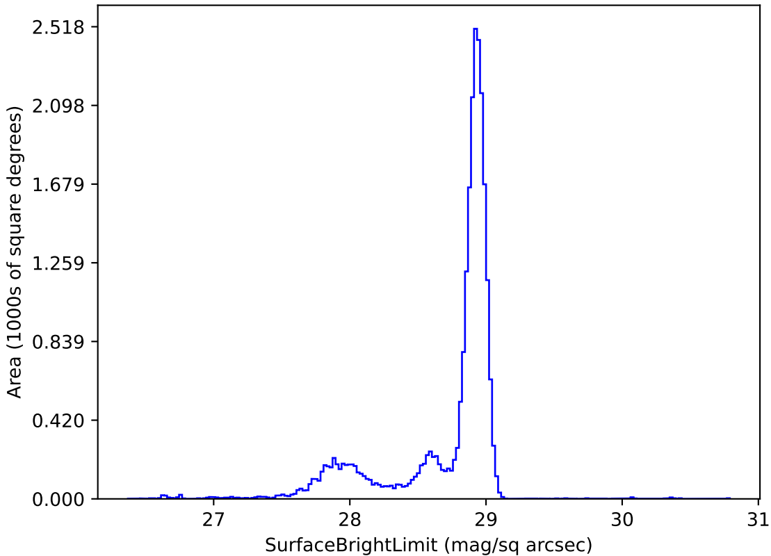
early_u_fpextra2.0_v3.4_10yrs u: SurfaceBrightLimit
