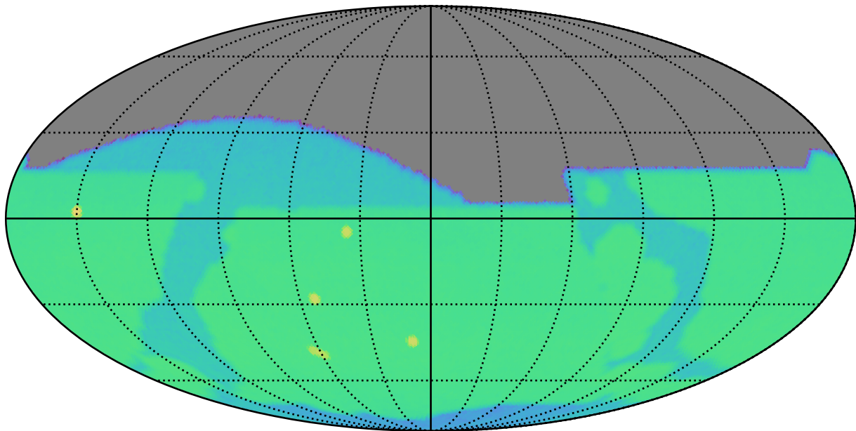
early_u_fpextra2.0_v3.4_10yrs r: SurfaceBrightLimit
