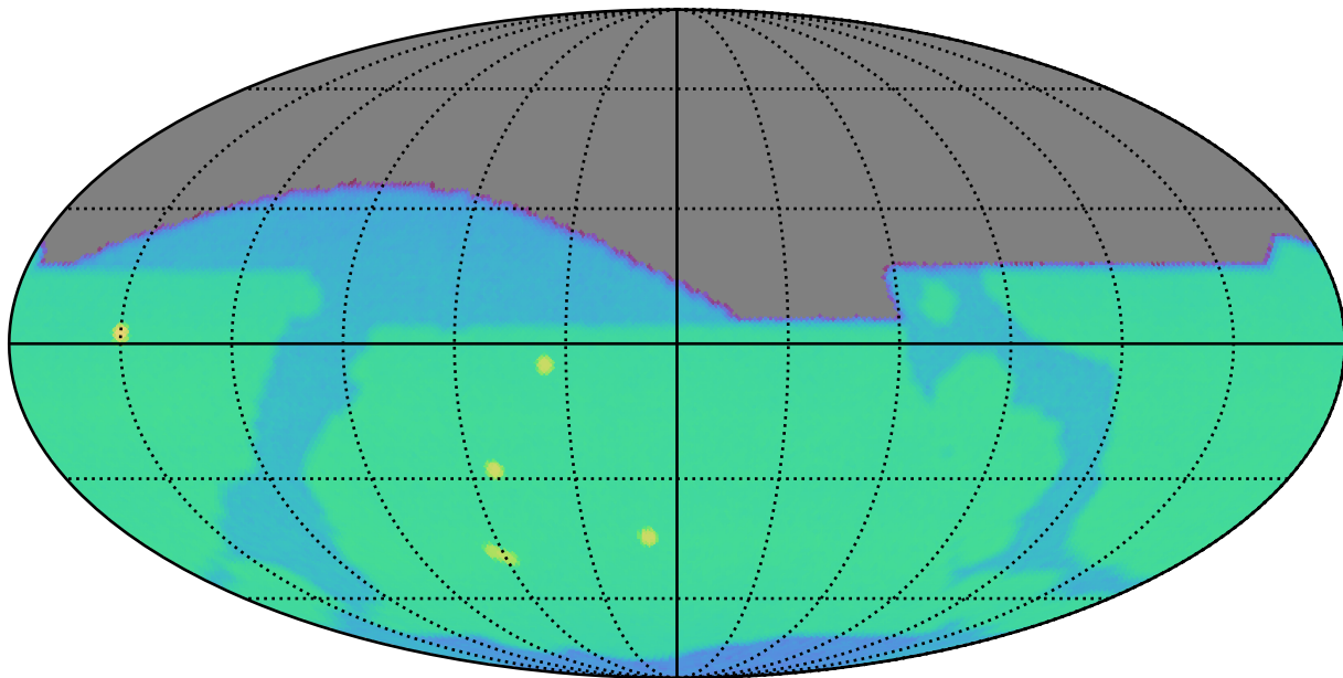
early_u_fpextra2.0_v3.4_10yrs i: SurfaceBrightLimit
