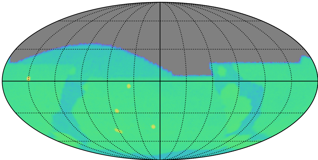
early_u_fpextra2.0_v3.4_10yrs g: SurfaceBrightLimit
