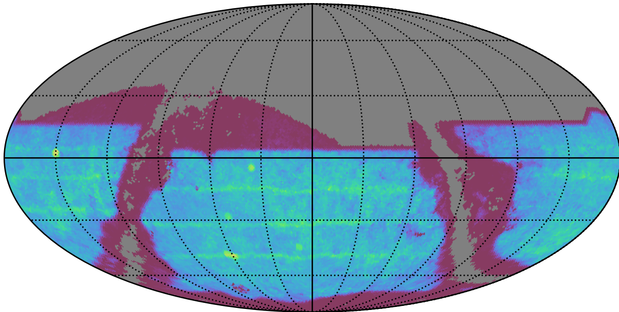
early_u_fpextra2.0_v3.4_10yrs : SNSLMetric
