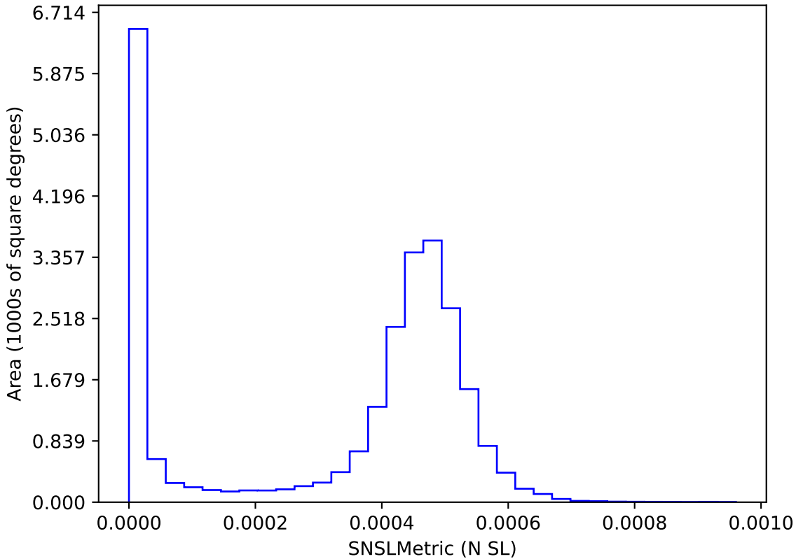
early_u_fpextra2.0_v3.4_10yrs : SNSLMetric
