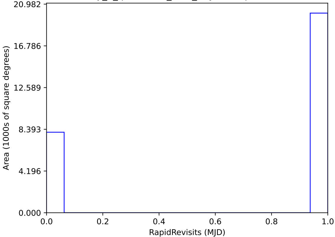
early_u_fpextra2.0_v3.4_10yrs : RapidRevisits
