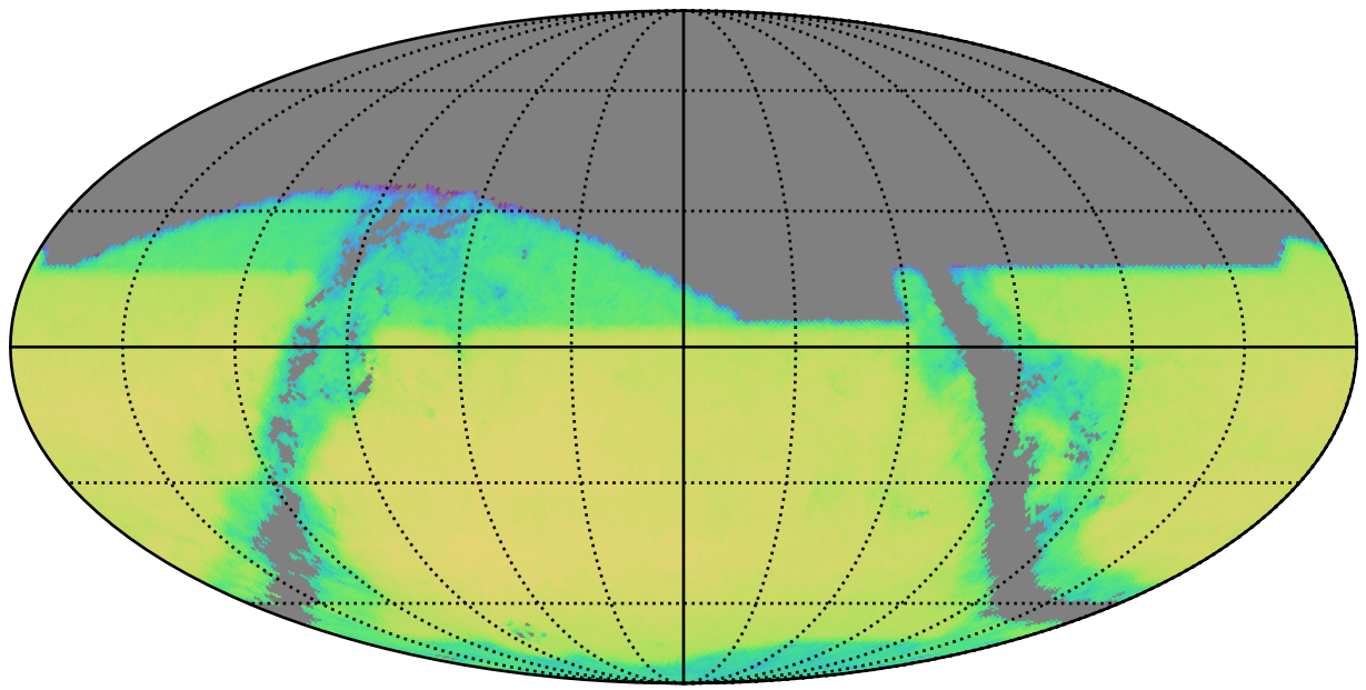
early_u_fpextra2.0_v3.4_10yrs z band and non-DD: QSONumberCountsMetric
