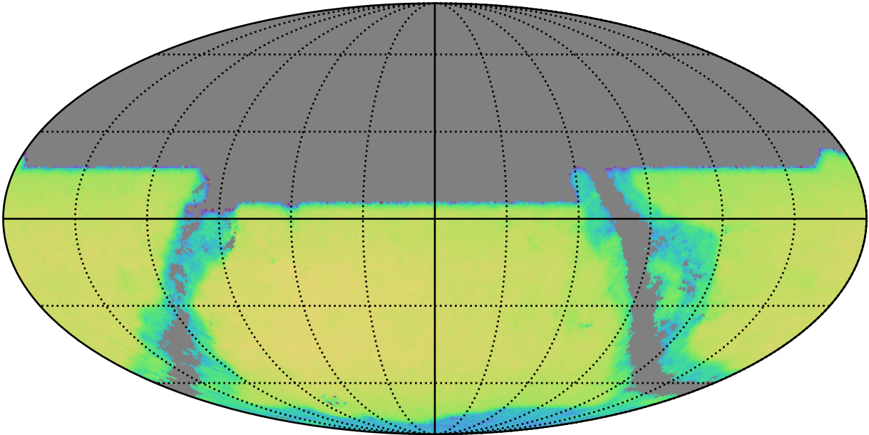
early_u_fpextra2.0_v3.4_10yrs y band and non-DD: QSONumberCountsMetric
