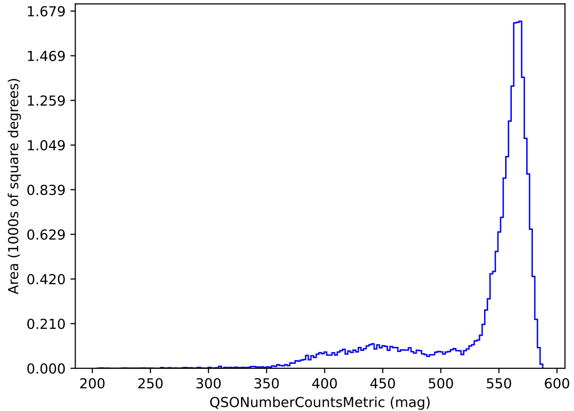
early_u_fpextra2.0_v3.4_10yrs y band and non-DD: QSONumberCountsMetric
