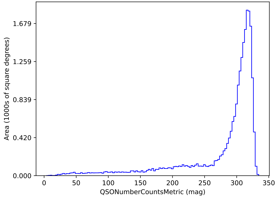
early_u_fpextra2.0_v3.4_10yrs u band and non-DD: QSONumberCountsMetric
