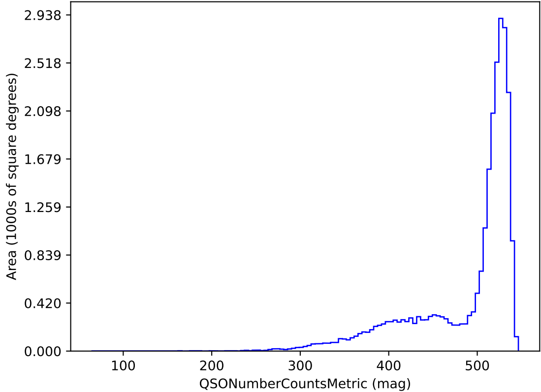
early_u_fpextra2.0_v3.4_10yrs r band and non-DD: QSONumberCountsMetric
