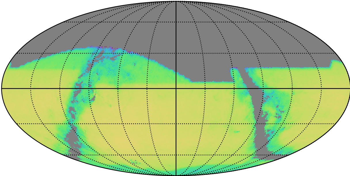
early_u_fpextra2.0_v3.4_10yrs i band and non-DD: QSONumberCountsMetric
