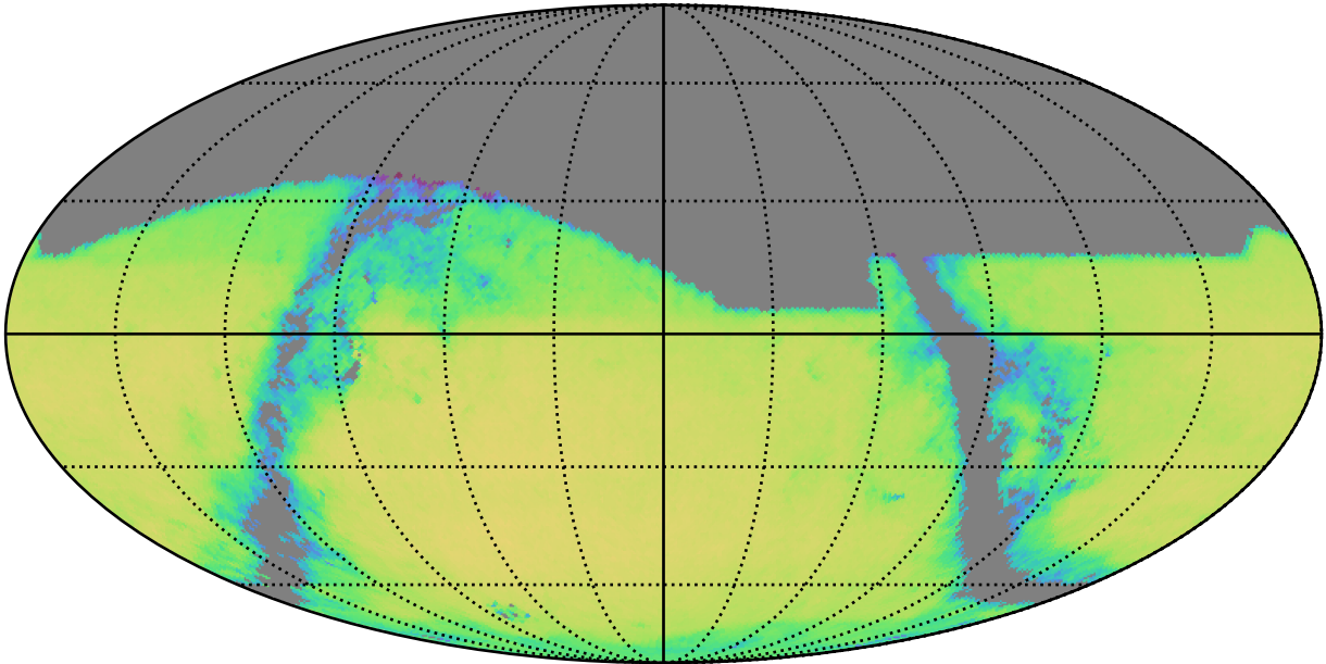
early_u_fpextra2.0_v3.4_10yrs g band and non-DD: QSONumberCountsMetric
