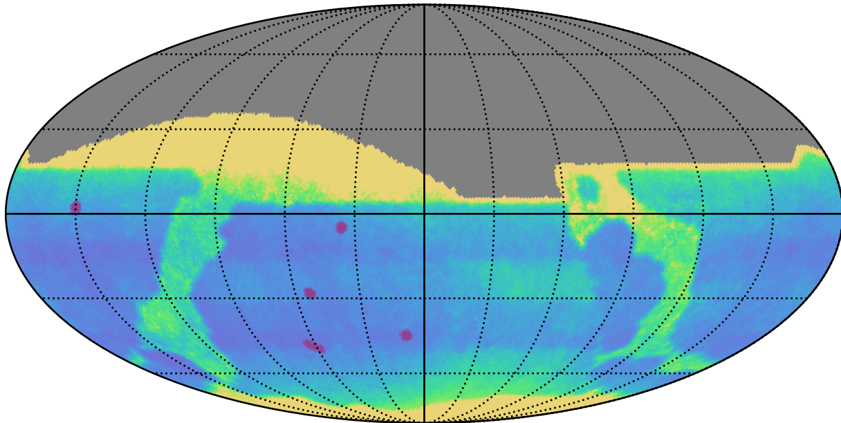
early_u_fpextra2.0_v3.4_10yrs : Proper Motion Uncert @ 24.0
