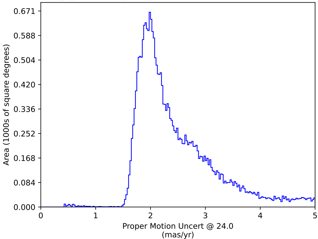
early_u_fpextra2.0_v3.4_10yrs : Proper Motion Uncert @ 24.0
