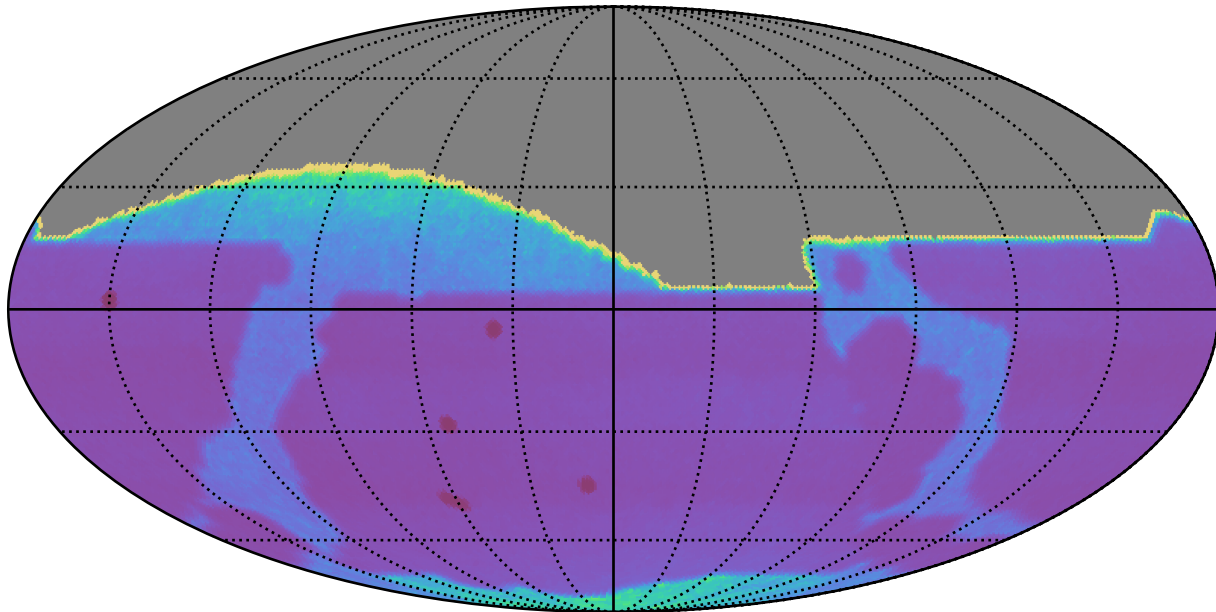
early_u_fpextra2.0_v3.4_10yrs : Proper Motion Uncert @ 20.5
