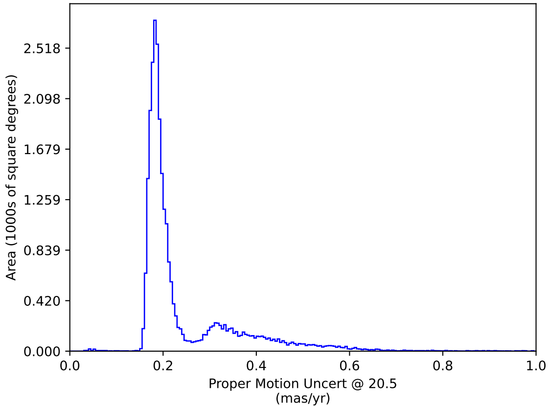
early_u_fpextra2.0_v3.4_10yrs : Proper Motion Uncert @ 20.5
