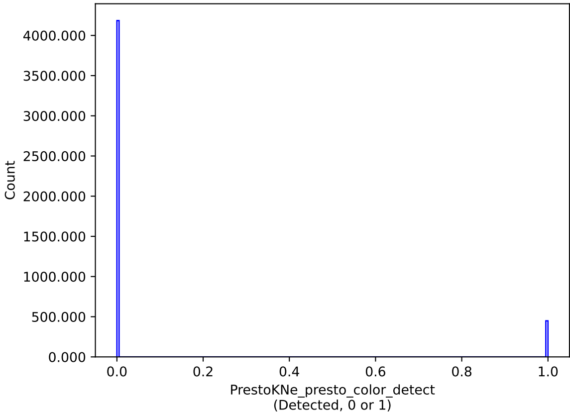
early_u_fpextra2.0_v3.4_10yrs : PrestoKNe_presto_color_detect
