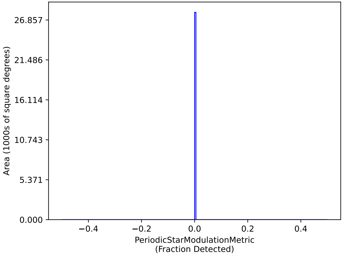
early_u_fpextra2.0_v3.4_10yrs dm 21 interval 15 RRC Year 1-2: PeriodicStarModulationMetric
