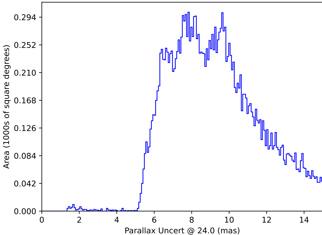
early_u_fpextra2.0_v3.4_10yrs : Parallax Uncert @ 24.0
