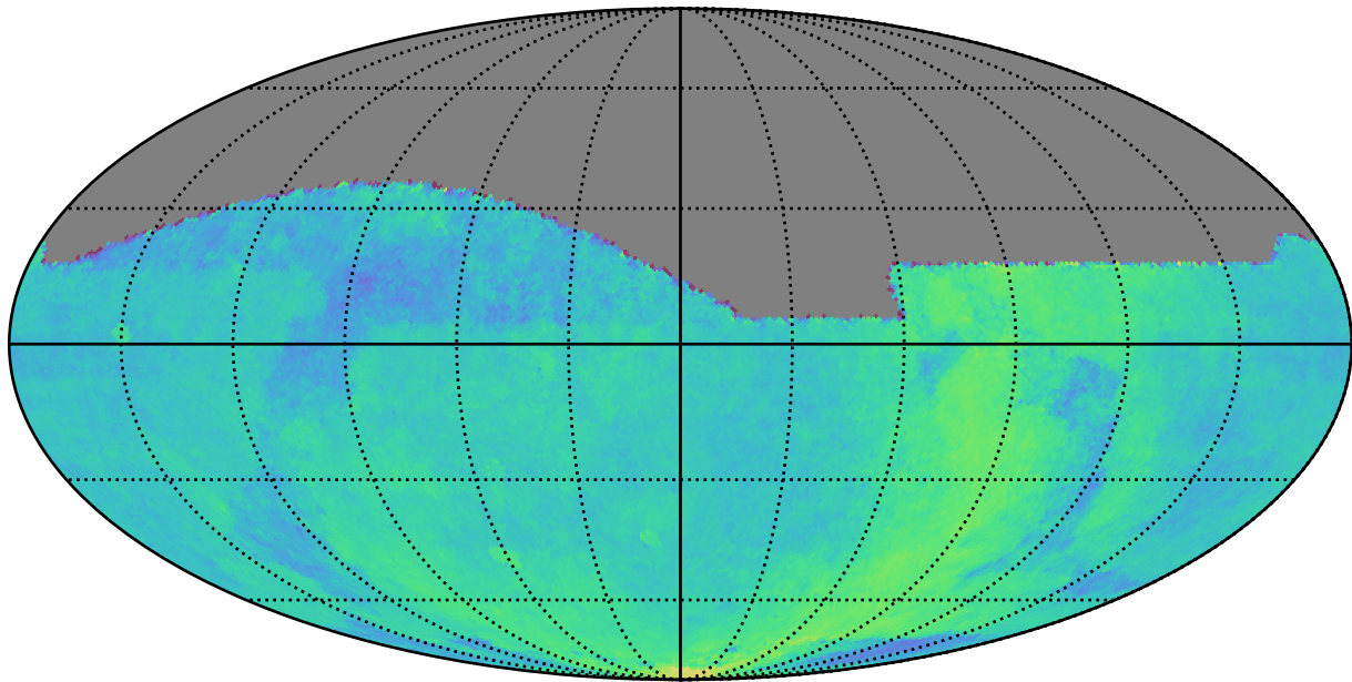
early_u_fpextra2.0_v3.4_10yrs : Parallax Coverage @ 24.0
