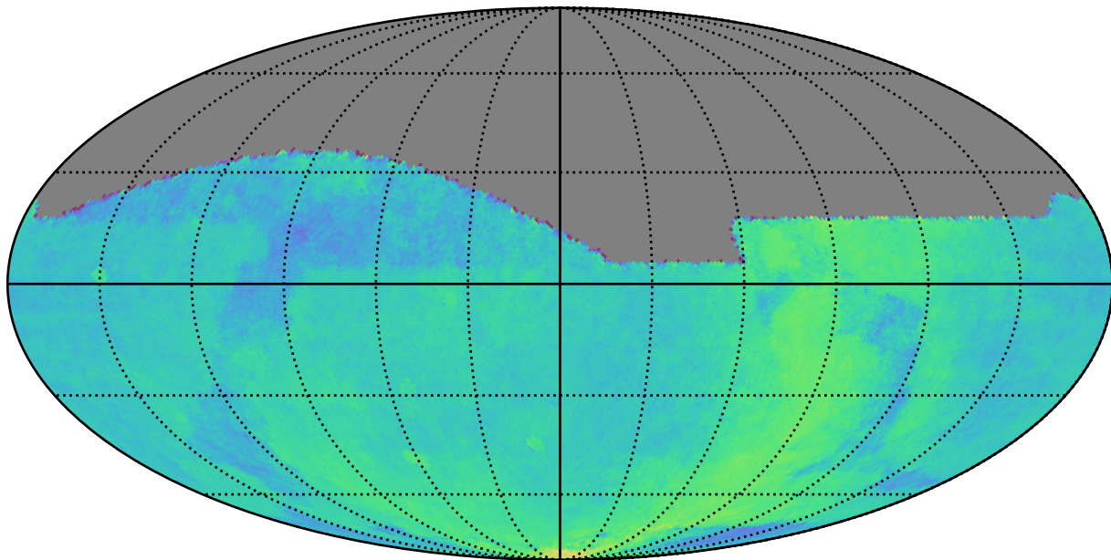
early_u_fpextra2.0_v3.4_10yrs : Parallax Coverage @ 22.4
