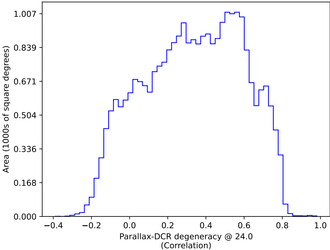
early_u_fpextra2.0_v3.4_10yrs : Parallax-DCR degeneracy @ 24.0
