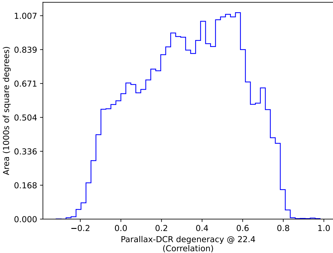
early_u_fpextra2.0_v3.4_10yrs : Parallax-DCR degeneracy @ 22.4
