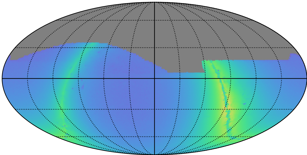
early_u_fpextra2.0_v3.4_10yrs z: Nstars_no_crowding
