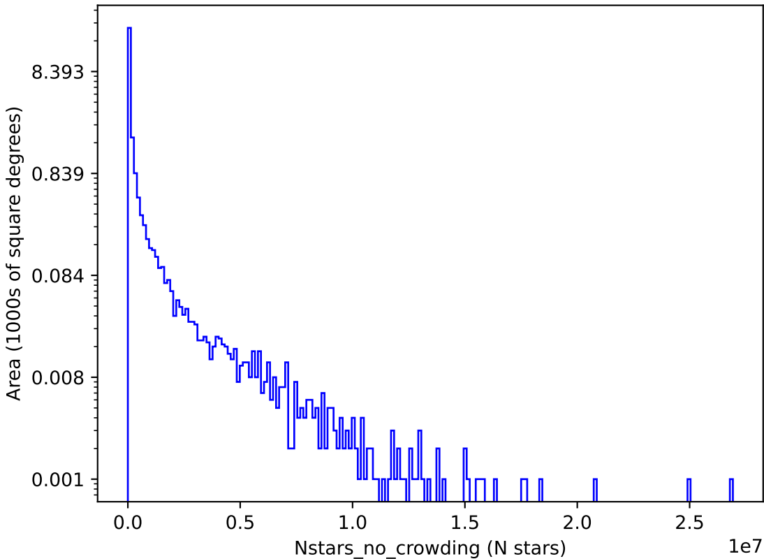
early_u_fpextra2.0_v3.4_10yrs z: Nstars_no_crowding
