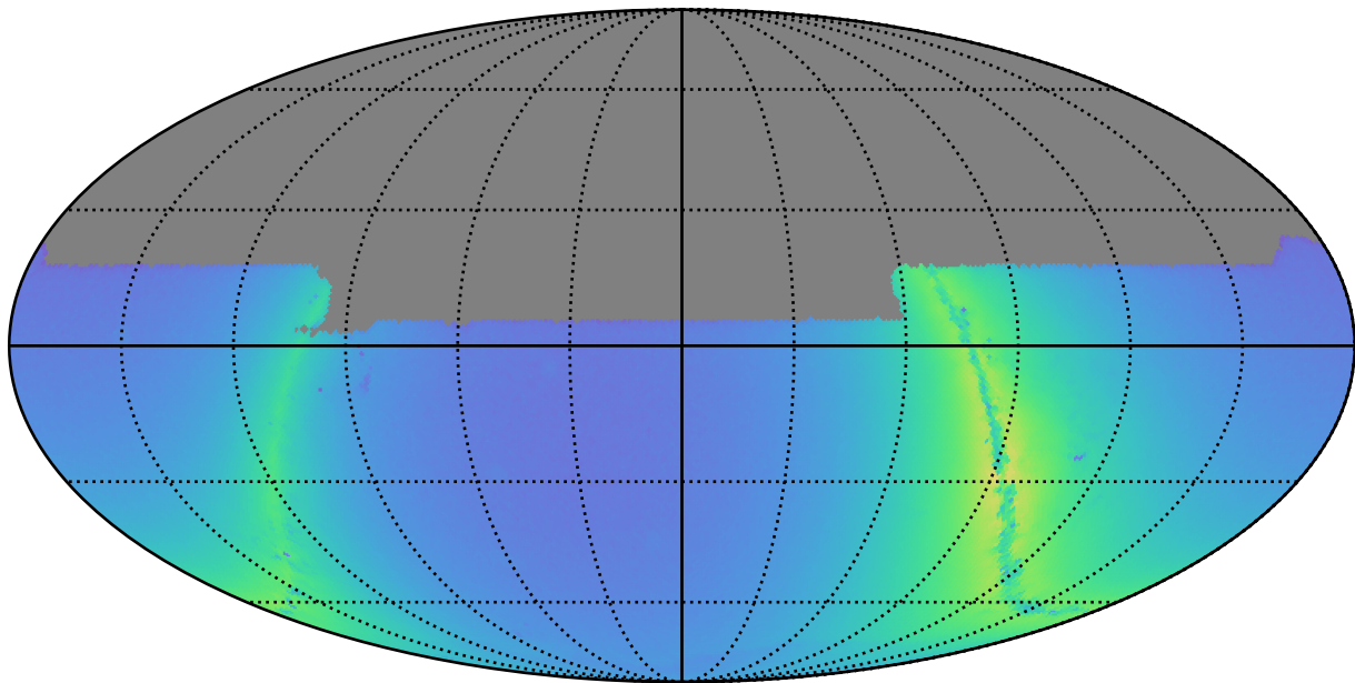
early_u_fpextra2.0_v3.4_10yrs y: Nstars_no_crowding
