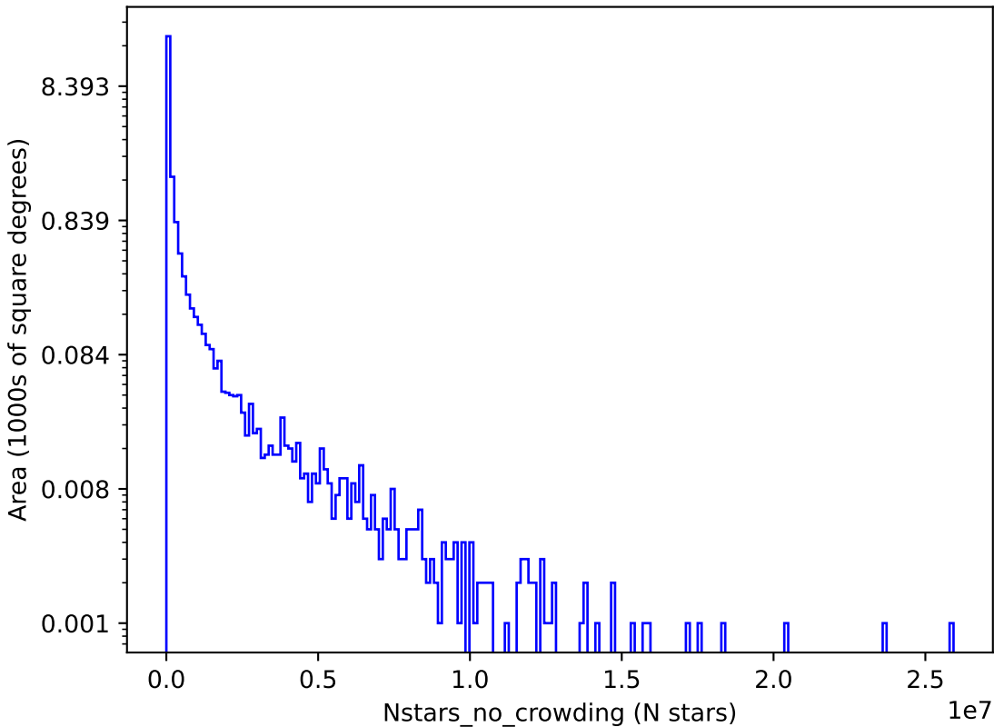
early_u_fpextra2.0_v3.4_10yrs y: Nstars_no_crowding
