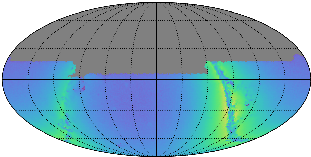
early_u_fpextra2.0_v3.4_10yrs u: Nstars_no_crowding
