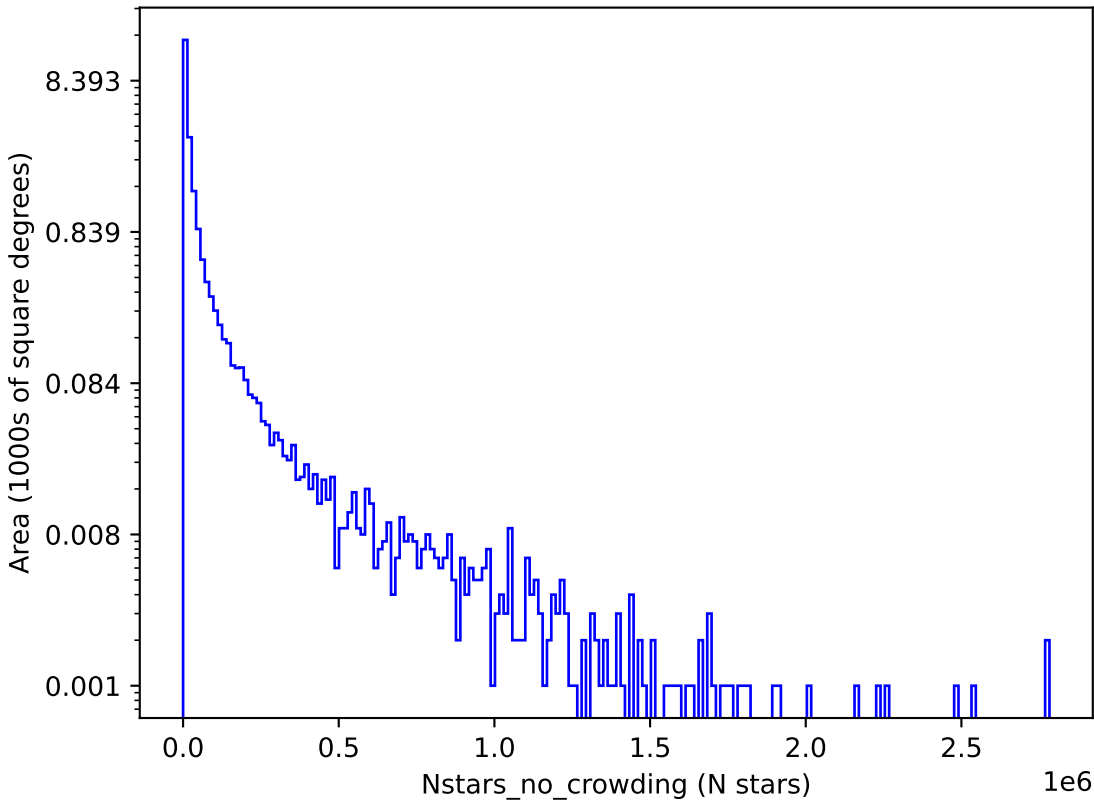
early_u_fpextra2.0_v3.4_10yrs u: Nstars_no_crowding
