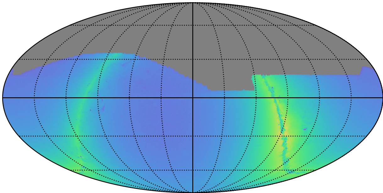
early_u_fpextra2.0_v3.4_10yrs r: Nstars_no_crowding
