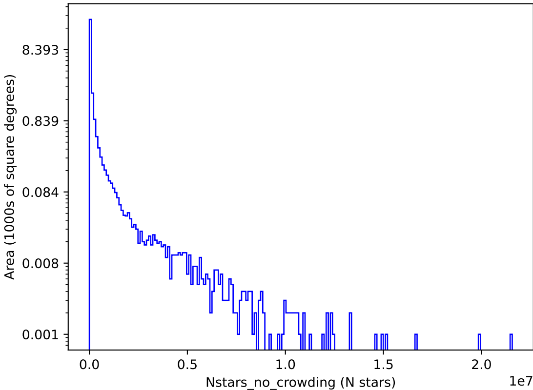
early_u_fpextra2.0_v3.4_10yrs r: Nstars_no_crowding
