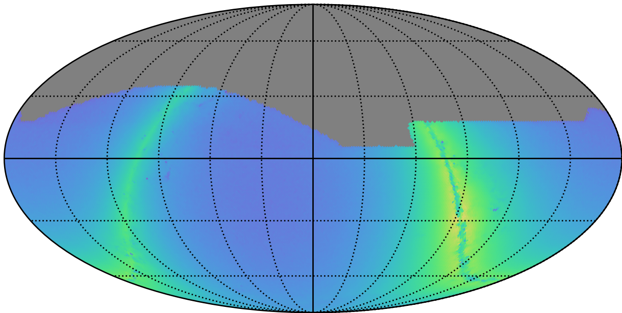
early_u_fpextra2.0_v3.4_10yrs i: Nstars_no_crowding
