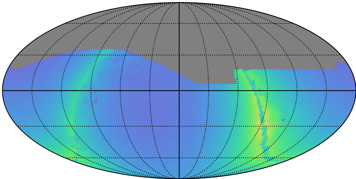
early_u_fpextra2.0_v3.4_10yrs g: Nstars_no_crowding
