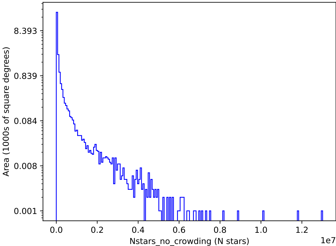
early_u_fpextra2.0_v3.4_10yrs g: Nstars_no_crowding
